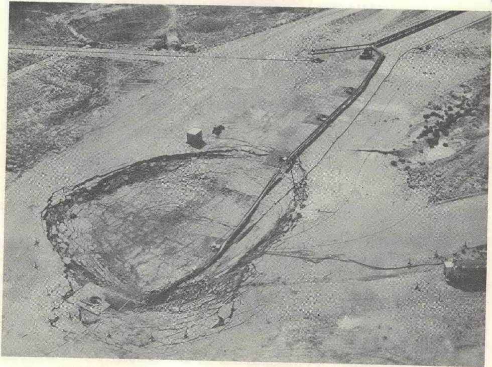
Fig. 9. Subsidence crater formed when the cavity collapsed. (View is to the southwest.) The square concrete block (left center of photo), now partly slumped into the crater, is the access-shaft pad. The shot point was directly below the north edge of the pad. The cable tray stretches from the pad along a path nine meters north of the tunnel. The crown block in the upper right corner lies directly above the end of the 122-meter tunnel. Along the cable tray are cable holes to the four instrument alcoves.
