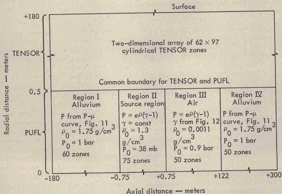
Fig. 10. Initial conditions used in Tensor-Pufl code for the numerical simulation of Marvel.
